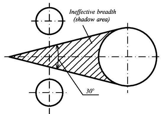
Fig. 1.4.8.3 Design section
