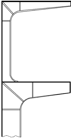
Fig. 3.1.2.10 Stiffening of cantilever beams
