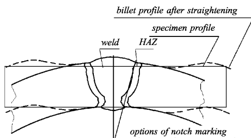
Fig. 5.3.4.4.2-2 Marking of pipe specimens
