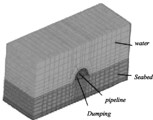
Fig. 4.1-2 Typical finite element model structure of the non-linear unburied subsea pipeline
