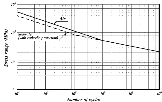
Fig. 5.5.7.4 S-N curve for pipeline welded joints
