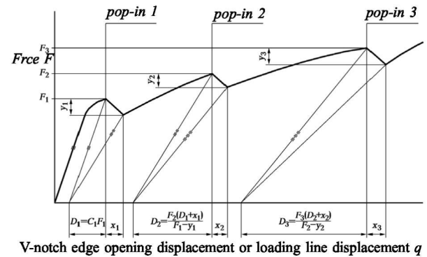
Fig. 2-3 The assessment procedure for pop-in significance on the deformation curve
