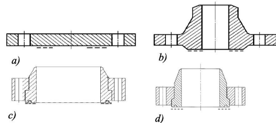
Fig. 4.7.3.4 Main types of flanges for subsea pipelines (the contact surface is shown with dashed line): a – blind flange; b – weldneck flange; c – swivel flange; d – swivel flange with profiled end face
