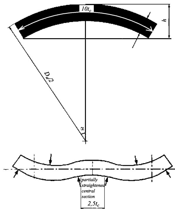
Fig. 2-1 Transverse pipe billet straightening
