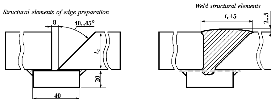
Fig. 5.2.1.2 Welded joints of rolled flat products for weldability tests
