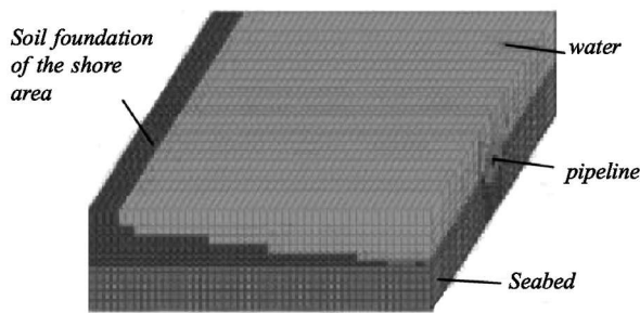
Fig. 4.1-1 Typical finite element model structure of the subsea pipeline shore approach
