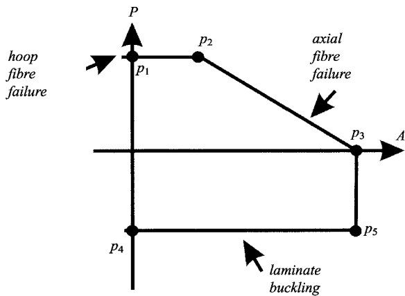
Fig. 1.3.4-3 Global failure envelope for composite riser pipe exposed to internal pressure and axial force
