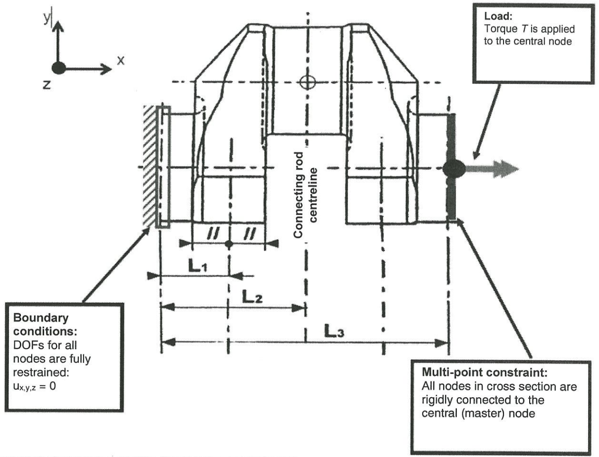
Fig. 3.1. Boundary and load conditions for torsion load case
