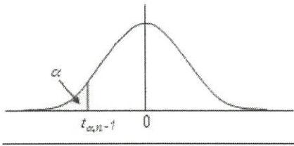
Fig. 2.5. Student's distribution
