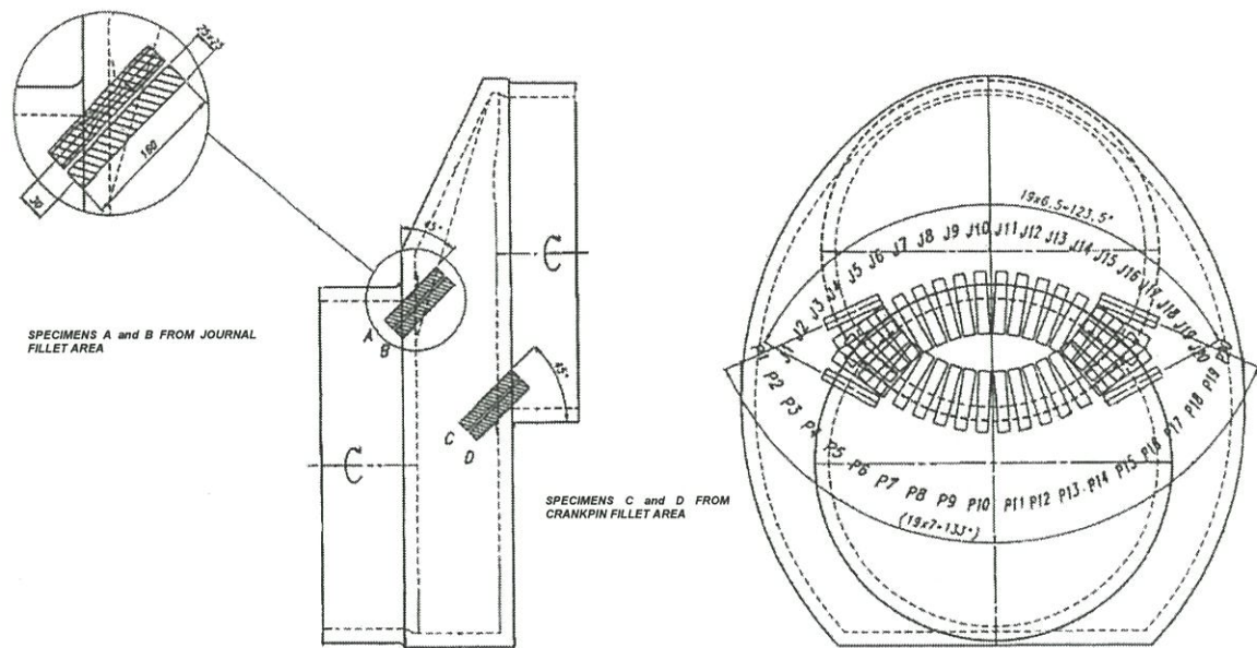
Fig. 3. Specimen locations in a crank throw
