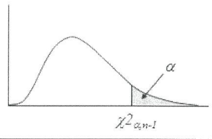
Figure 2.6. Chi-square distribution
