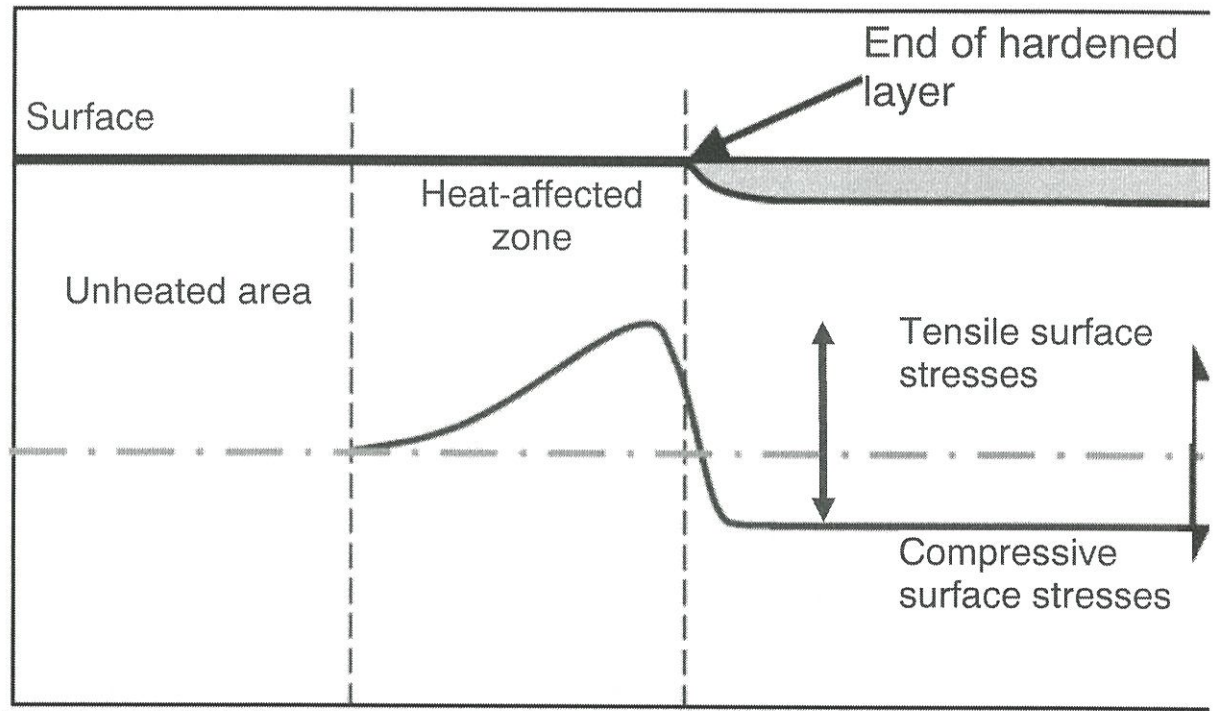
Fig. 4-2. Residual stresses along the surface of a crankpin and fillet
