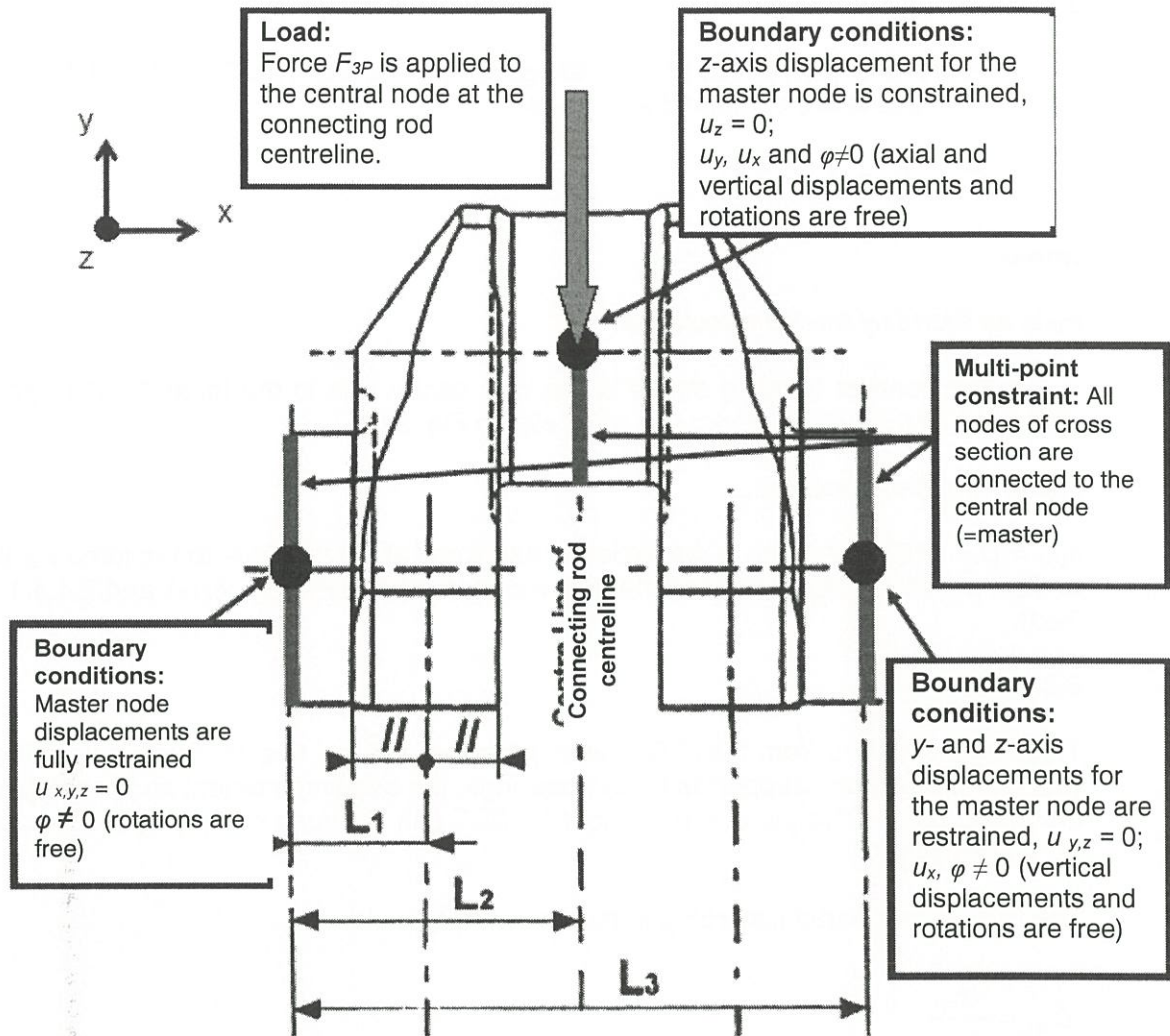
Fig. 3.3. Boundary and load conditions for 3-point bending load case of in-line engine.
