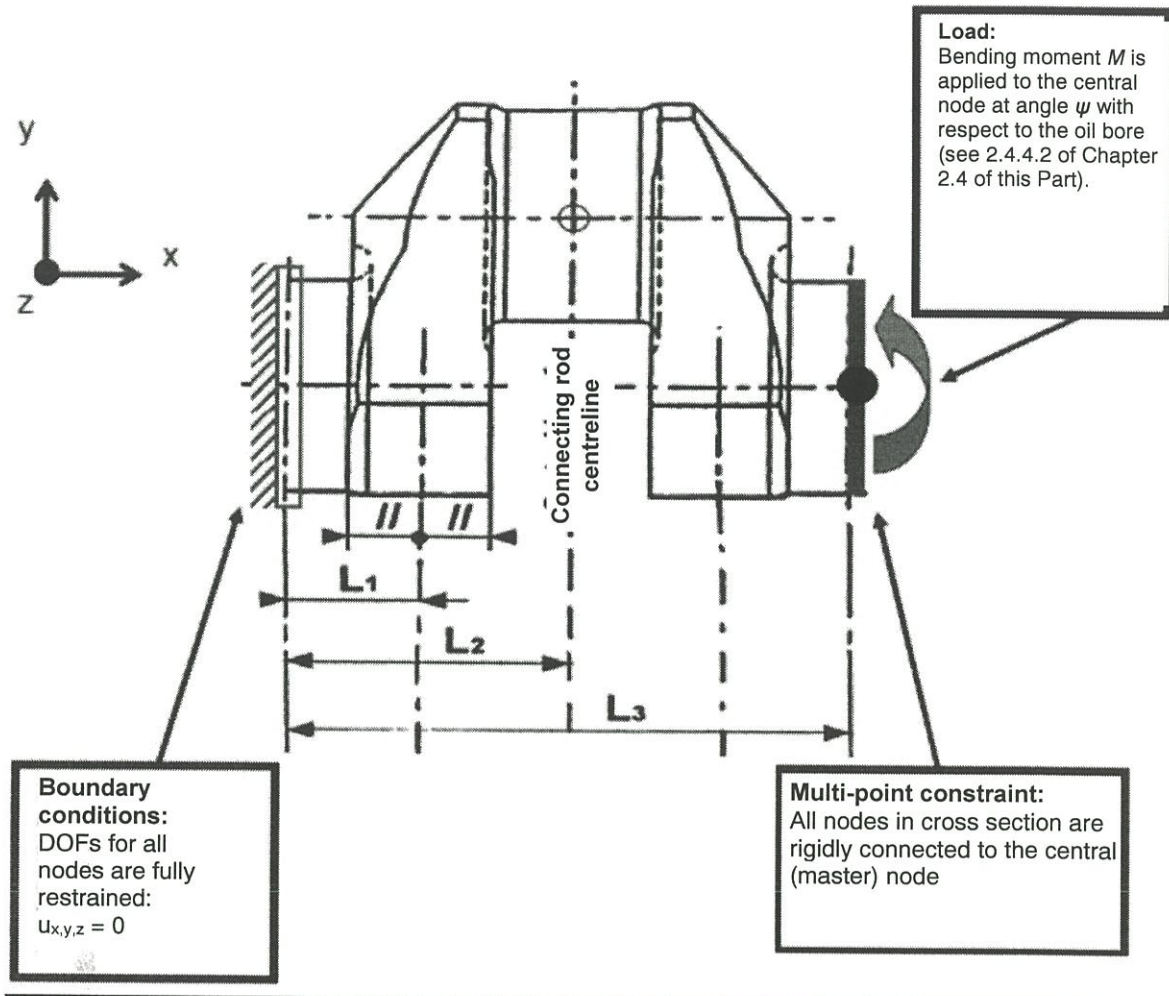
Fig. 3.2. Boundary and load conditions for pure bending load case
