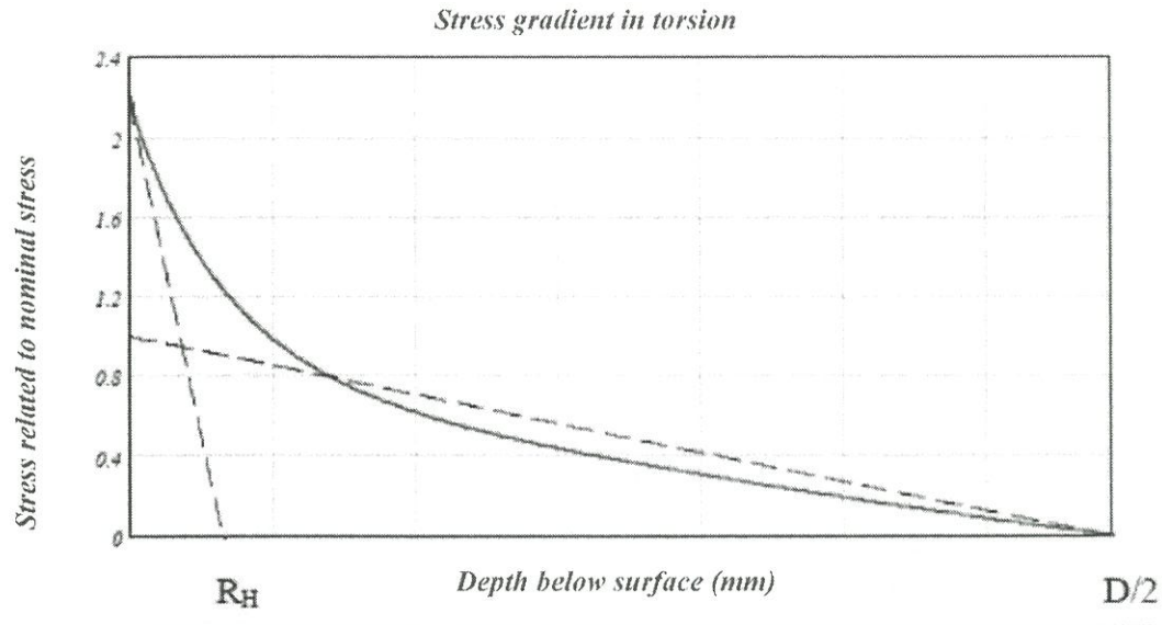
Fig. 3.1-2. Torsional SCF in crankpin fillet as a function of depth. The corresponding SCF for the journal fillet can be found by replacing R_H with R_G and D with D_G
