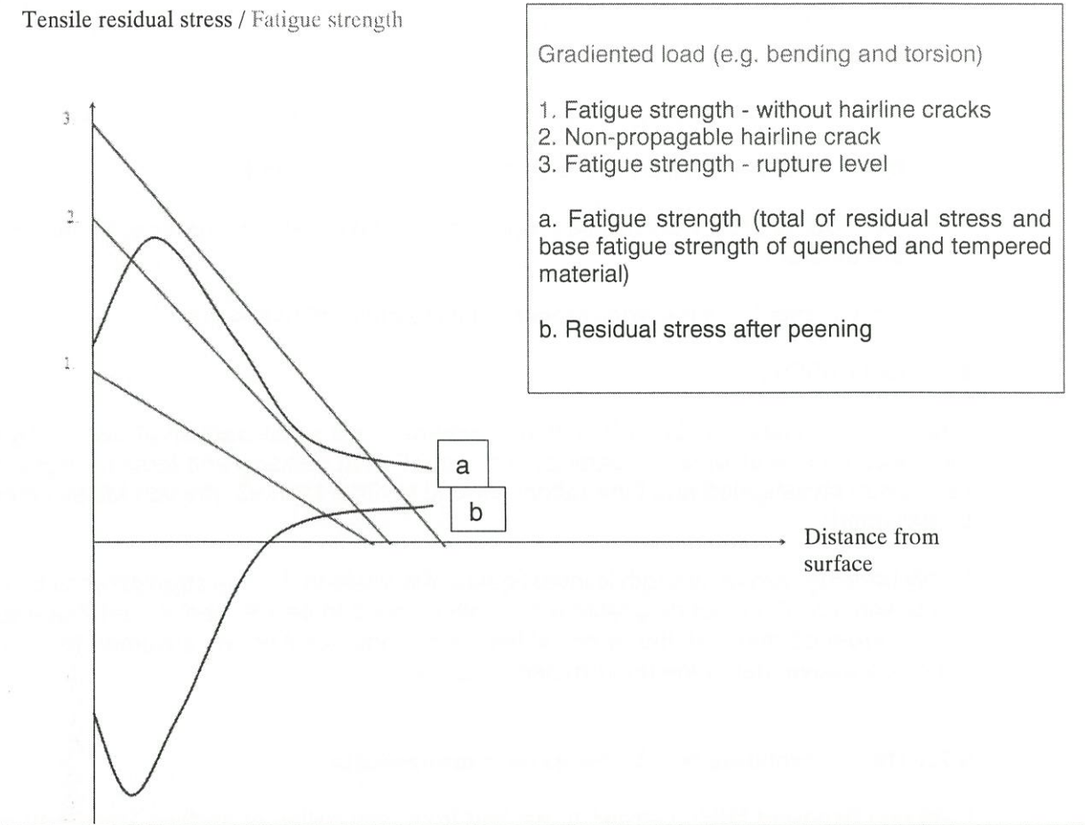
Fig. 6.1. Working and residual stresses below the stroke-peened surface. Straight lines 1 to 3 represent different possible load stress gradients
