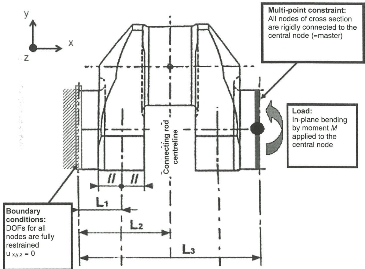
Fig. 3.2. Boundary and load conditions for pure bending load case
