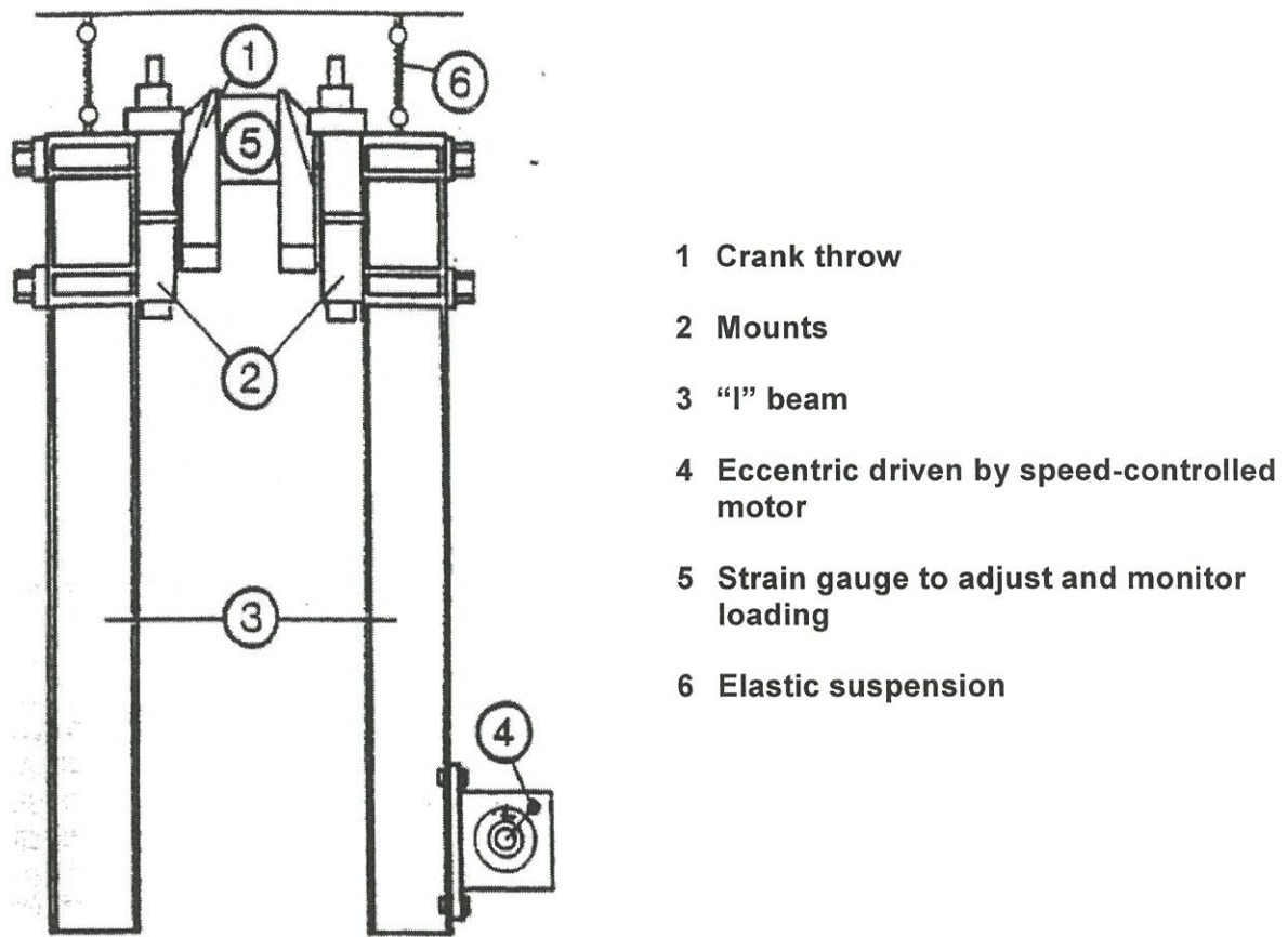
Fig. 4.2-1. An example of resonance test rig setup for bending loading test
