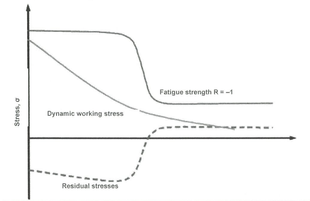
Fig. 3. Stresses as functions of depth, general principles
