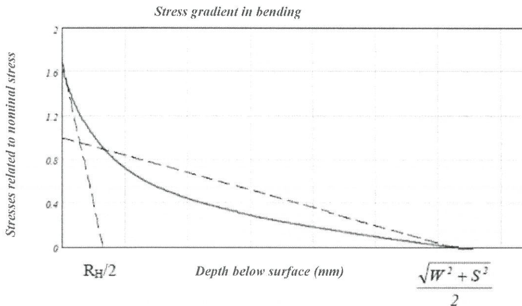
Fig. 3.1-1. Bending SCF in crankpin fillet as a function of depth. The corresponding SCF for the journal fillet can be found by replacing R_H with R_G
