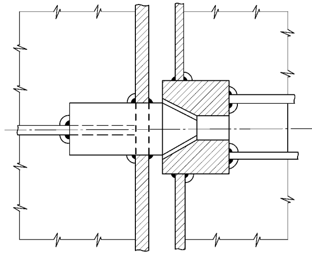
Fig. 7.4.2.8 Thrust bearing
