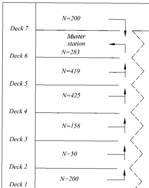
Fig. 3-1 Minimum stairway width calculation example:
