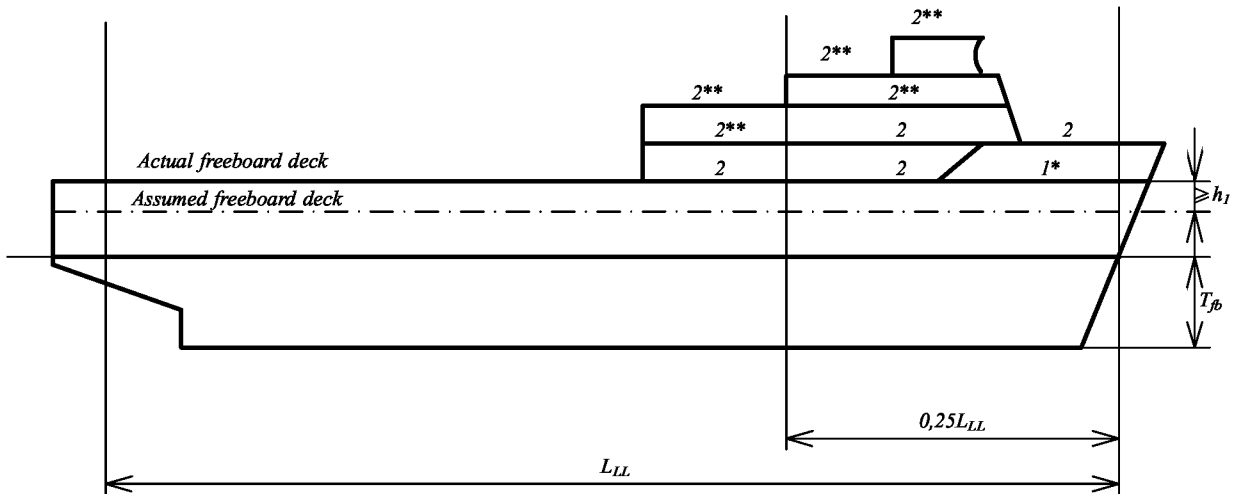
Positions 1 and 2 for an increased freeboard
