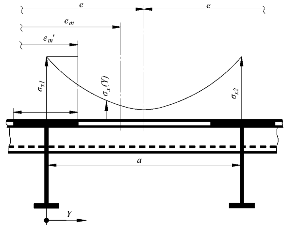
Fig. 7.10.6.29-2 Stiffening perpendicular to web of primary supporting member
