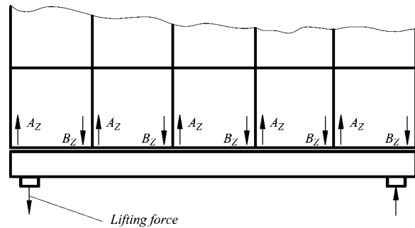
Fig. 7.10.6.48 Lifting forces at a hatch cover
