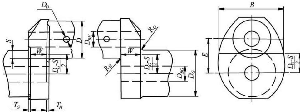
Fig. 2.4.6.1-1 Crank dimensions necessary for the calculation of stress concentration factors:
