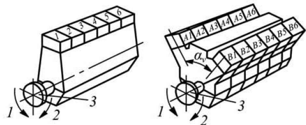
Fig. 2.4.3-1 Sense of crankshaft rotation: 1 — counter-clockwise; 2 — clockwise; 3 — driving shaft flange
