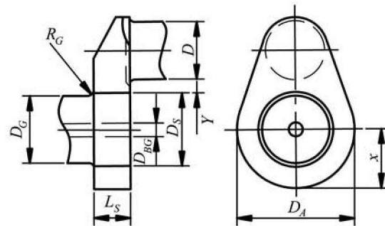
Fig. 2.4.10.1 Crank throw of semi-built crankshaft:
