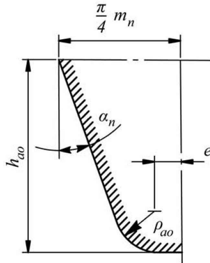
Fig. 4.2.2.7.3.2-2 Non-protuberance hob
