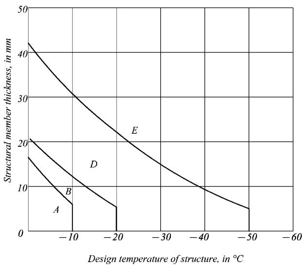
Fig. 1.2.3.1-3 Structural members of Class III
