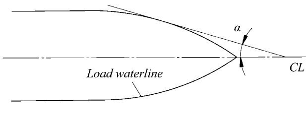
Fig. 3.10.1.2-1: \alpha — slope of summer load waterline at the section considered, in deg.
