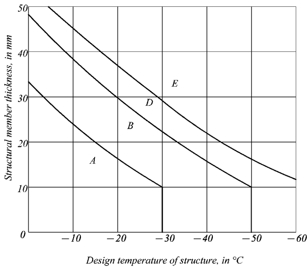
Fig. 1.2.3.1-1 Structural members of Class I
