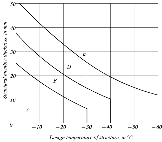
Fig. 1.2.3.1-2 Structural members of Class II
