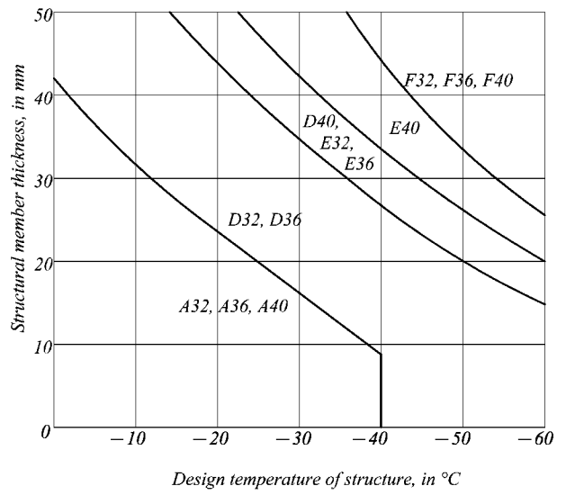
Fig. 1.2.3.1-1 Structural members of Class I
