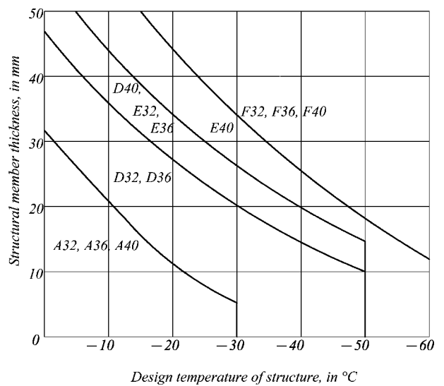
Fig. 1.2.3.1-3 Structural members of Class III
