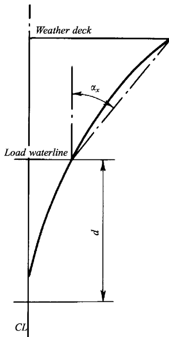
Fig. 2.8.1.2-1 Determination of angle \alpha_x
