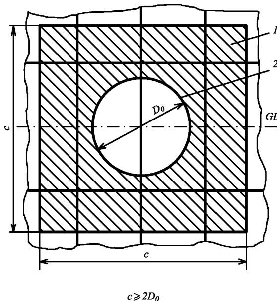
Fig. 3.6.4.12.5: 1 — thickened plate; 2 — tub
