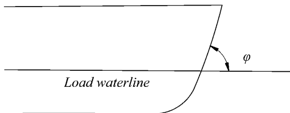
Fig. 3.10.1.2-4: \varphi — slope of stem on the level of summer load waterline, in deg.
