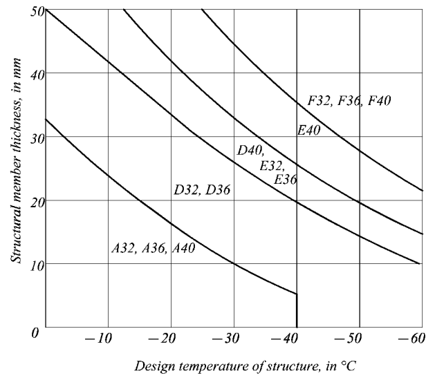
Fig. 1.2.3.1-2 Structural members of Class II
