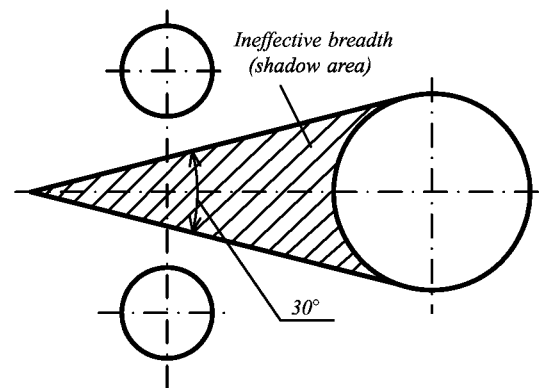
Fig. 1.4.8.3 Design section
