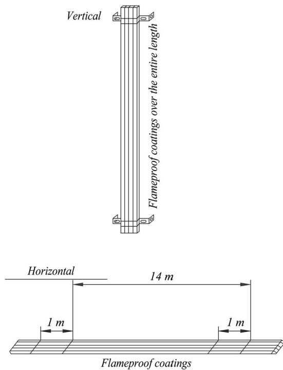
Fig. 16.8.4.3.2-1 Cable runs protected with flameproof coatings
