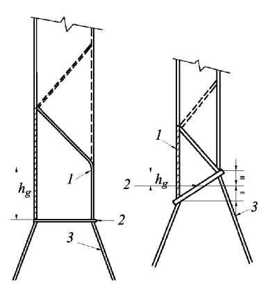
Fig. 4.2-4 Asymmetric gasset/shedder plates: 1 — gasset/shedder plate; 2 — top of the lower stool; 3 — vertical or sloping stool side plating
