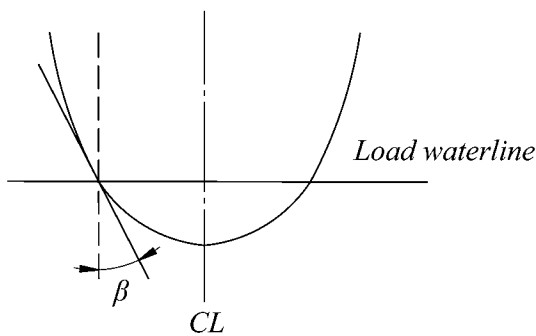
Fig. 3.10.1.2-2: \beta — slope of frame on the level of summer load waterline at the section considered, in deg.
