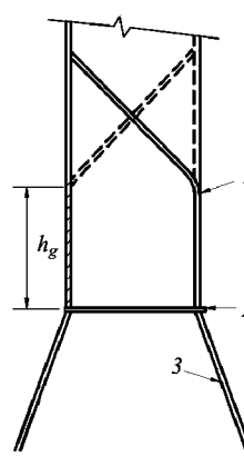
Fig. 4.2-3 Symmetric gasset/shedder plates: 1 — gasset/shedder plate; 2 — top of the lower stool; 3 — vertical or sloping stool side plating
