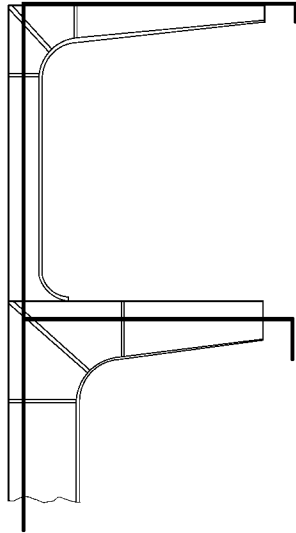
Fig. 3.1.2.10 Stiffening of cantilever beams
