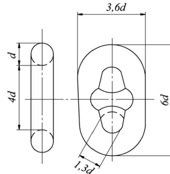
Fig. 7.1.3-1 Common link
