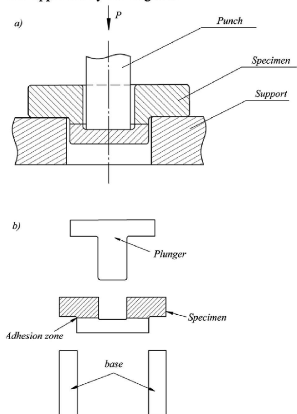
Fig. 5.3.2.3.4.3.2-1 Pull-off test diagrams (a or b)
