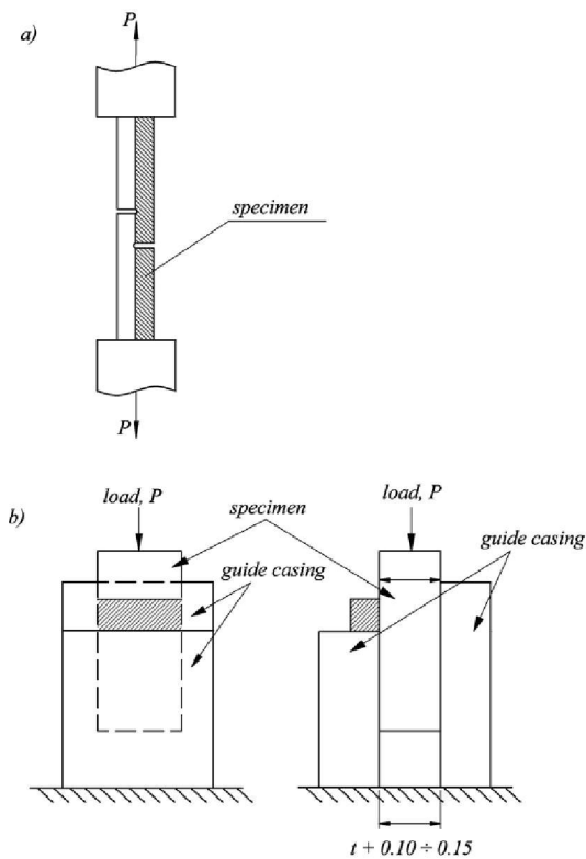
Fig. 5.3.2.3.4.3.2-2 Shear test diagrams (a or b)
