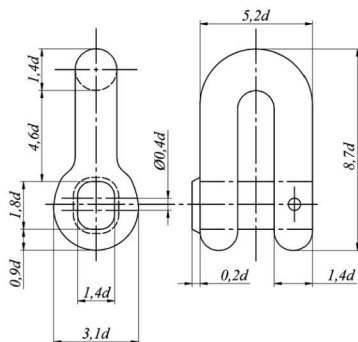
Fig. 7.1.3-6 End shackle
