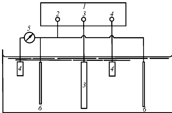
Fig. 2.5.6.1-1 Cathode protective circuit with potentiostatic control: 1 – potentiostat; 2 – work electrode; 3 – anode; 4 – reference electrode; 5 – voltmeter; 6 – test specimen
