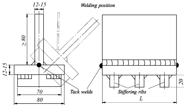
Fig. 4.2.4.1 Tee-joint test assembly for hot cracking test of welded joint: L = 120 mm — for manual welding with covered electrodes; L = 250 mm — for semiautomatic metal-arc electrode welding; L = 200 mm — for manual inert-gas tungsten-arc welding
