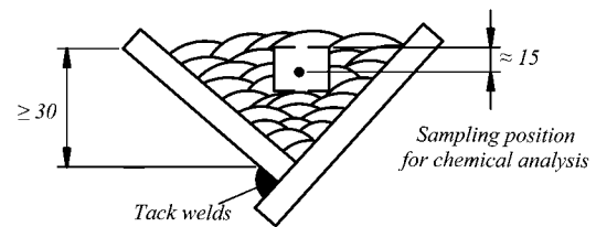
Fig. 4.9.2 Deposited metal test assembly
