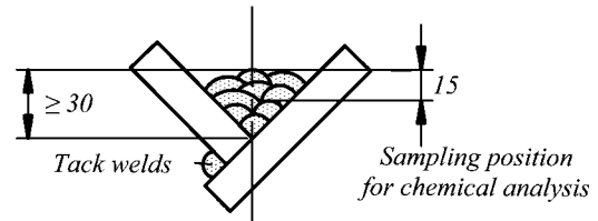
Fig. 4.10.2 Deposited metal test assembly
