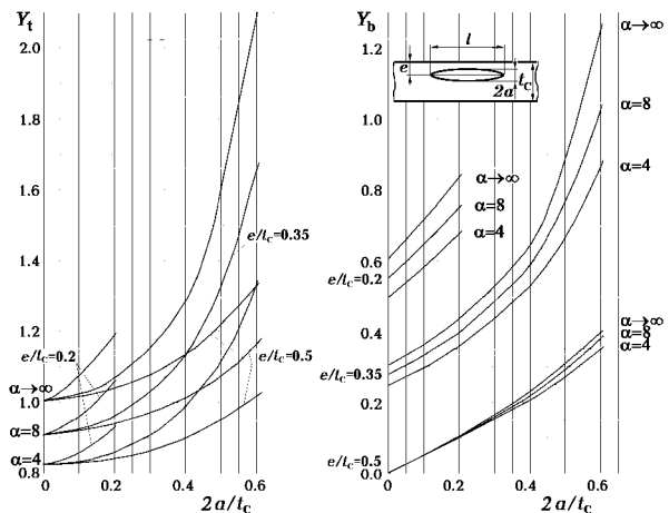
Nomographs for determination of Y-functions (surface semi-elliptic crack)
