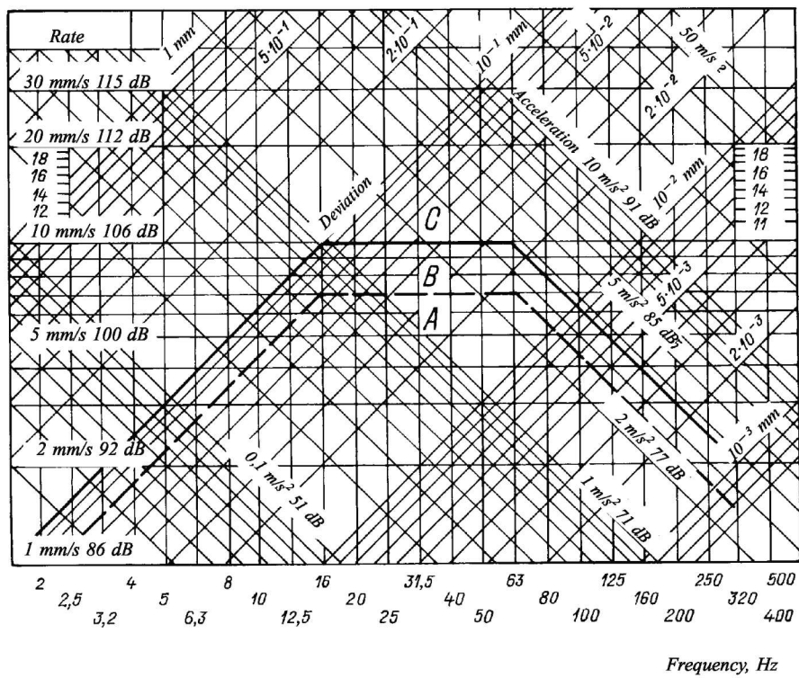
Fig. 9.5.1 Vibration standards for pumps with the capacity of 15 to 75 kW:
