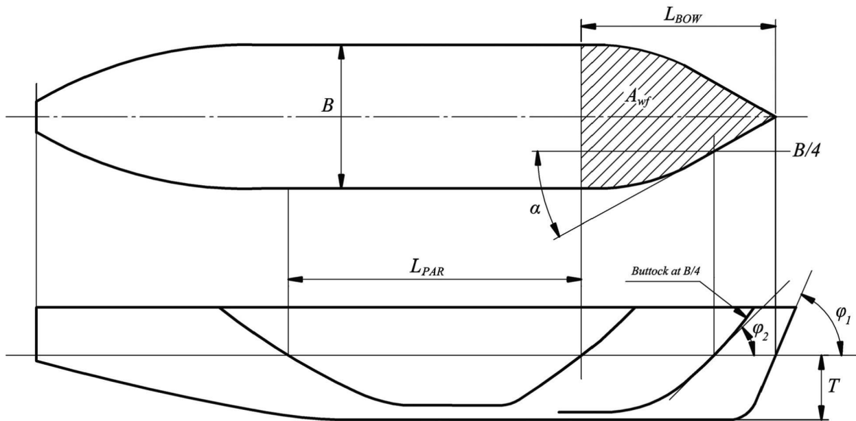
Fig. 2.1.1.4 Geometrical features of the ship for determination of the power delivered to the propeller shaft of ice class ships
