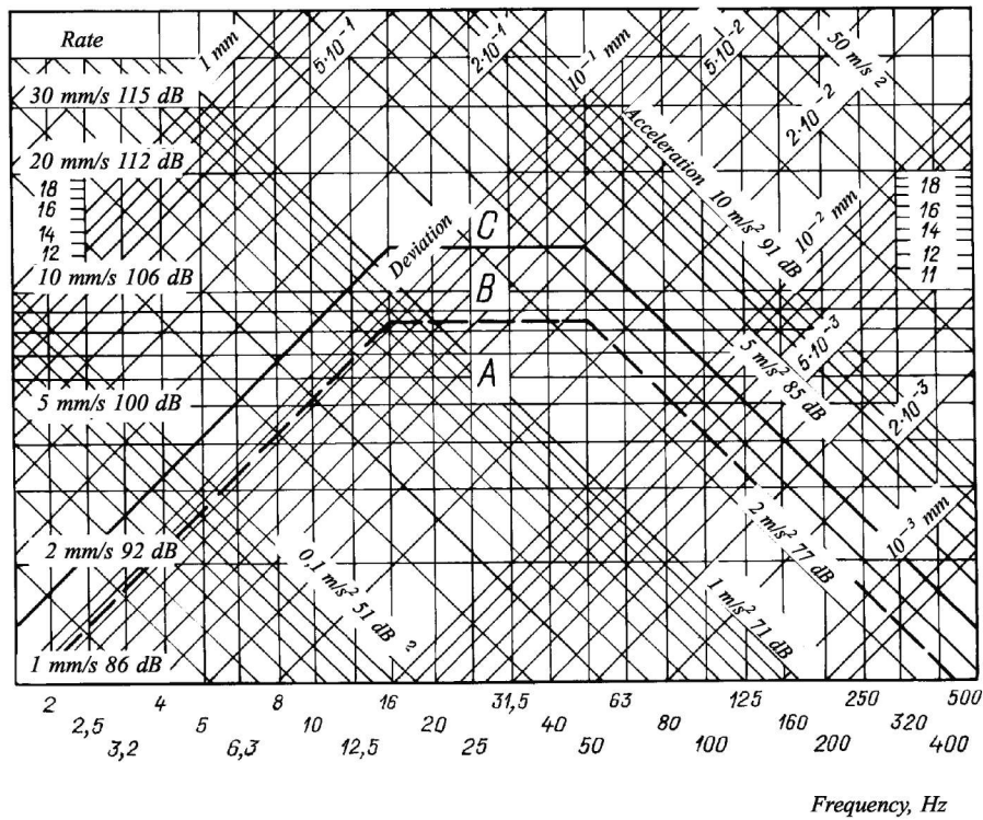
Fig. 9.5.3 Vibration standards for fans:
