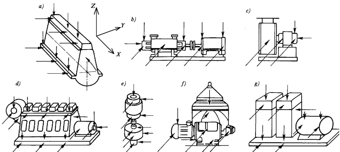
Fig. 9.2.5 Points of vibration measuring: a — internal combustion engine; b — horizontal pump; c — fan; d — diesel-generator; e — vertical pump; f — separator; g — piston compressor. The points and directions of vibration measurement are shown by arrows
