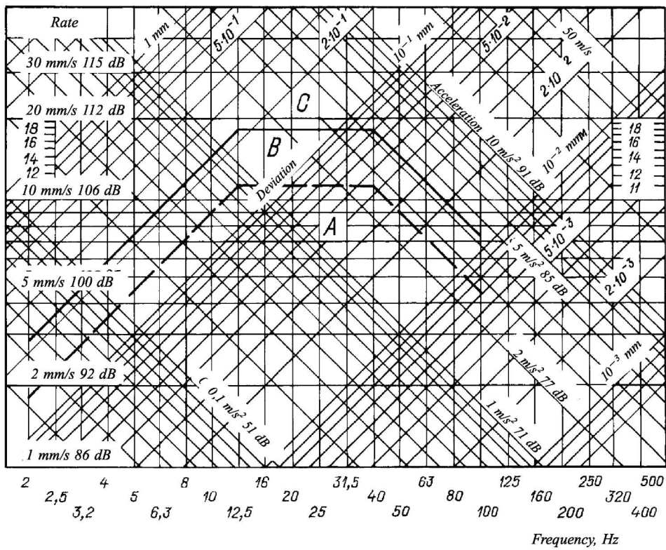
Fig. 9.4.1 Vibration standards for main steam geared turbines of 15000 to 30000 kW capacity and thrust bearings: - - - - - Upper limit of category A; ———— Upper limit of category B
