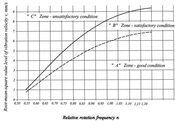
Fig. 9.9.3 Vibration standards of azimuth thrusters
