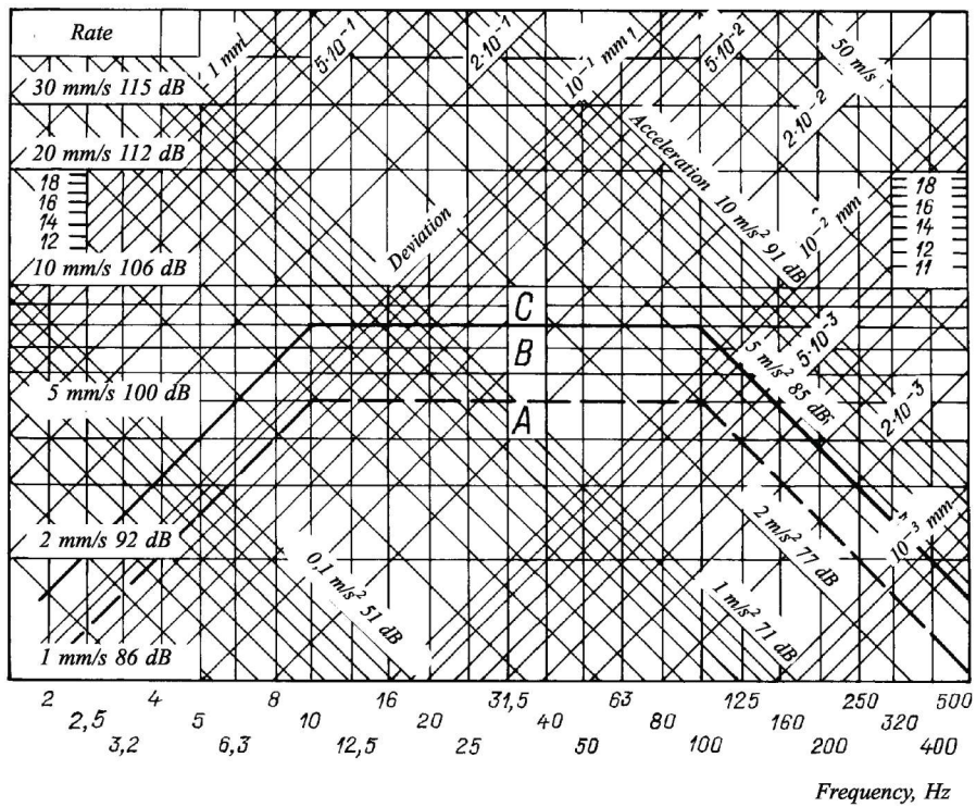
Fig. 9.5.2 Vibration standards for centrifugal separators:
