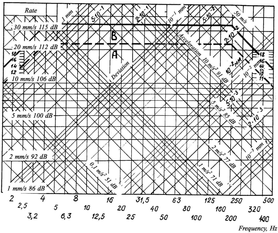
Fig. 9.3.4 Vibration standards for turbo-compressors of internal combustion engines: - - - - - Upper limit of category A; ———— Upper limit of category B
