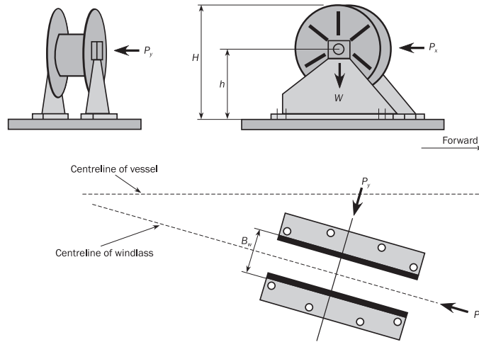
Figure 1 : Directions of forces and weight
