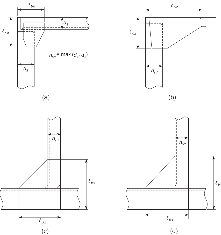
Figure 3 : Bracket arm length of non-continuous stiffeners
