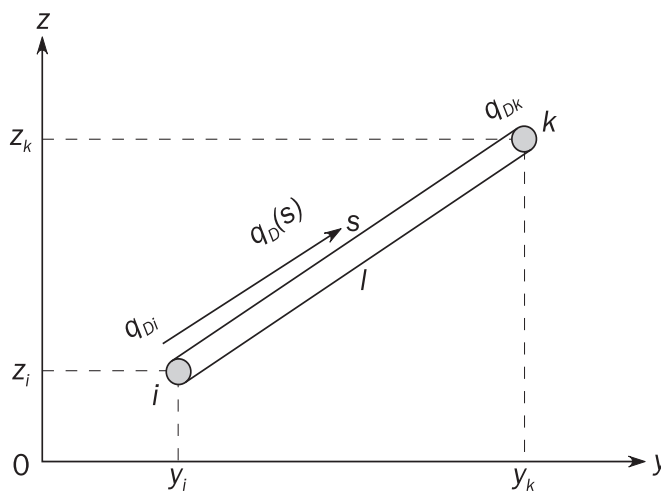
Figure 2 : Calculation of determinate shear flow at bifurcation
