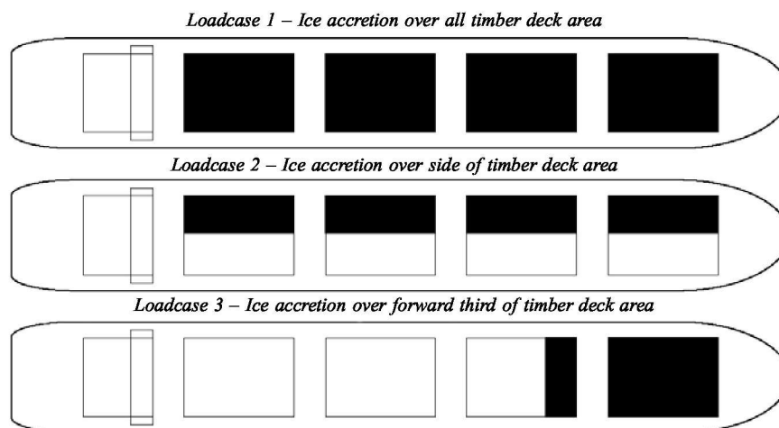
Fig. 3.3.7.3 Ice accretion load cases for timber deck cargoes
