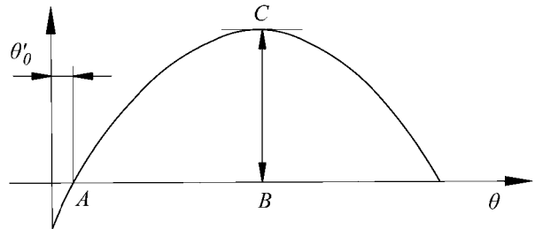
Fig. 1.3 Determination of capsizing moment in non-working condition
